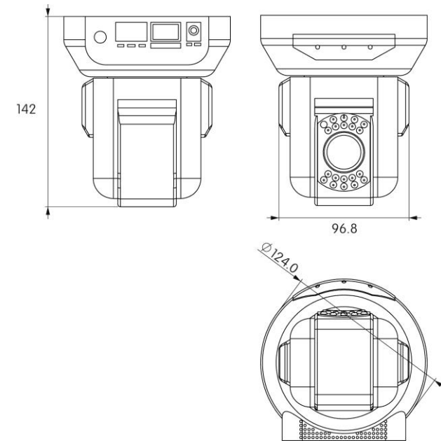
Dimension (mm)
